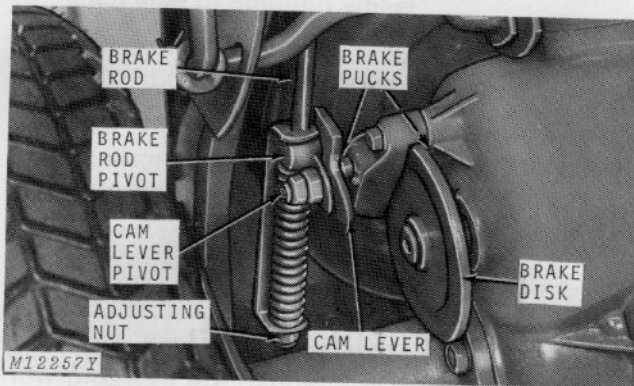
Bottom View—Right-Hand Side of Transaxle
