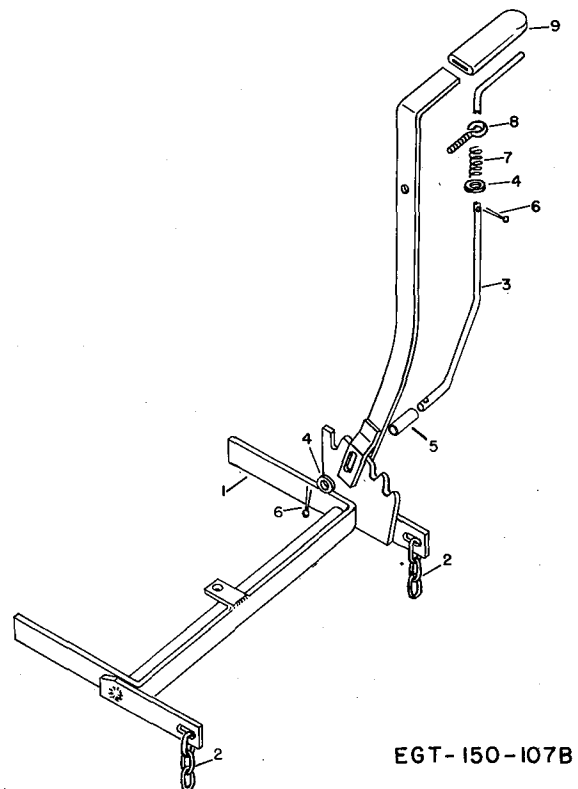
MANUAL REAR LIFT FOR EGT 120 - 150 EGT 200
