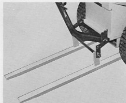
LIGHT DUTY PALLET HANDLER—REAR OR FRONT MOUNT CP20
